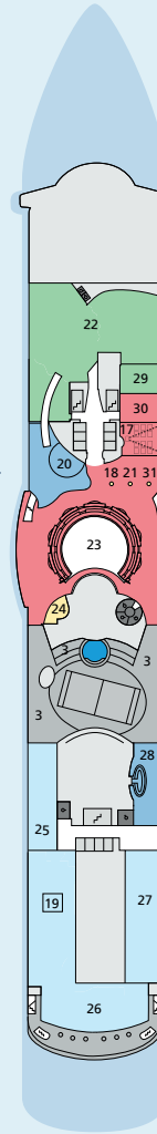
Deck 11
